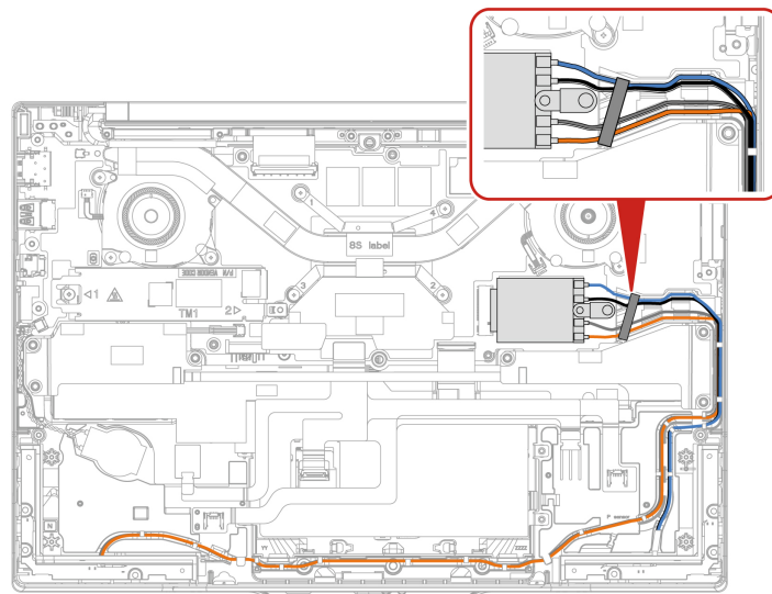
Type three – 5G wireless WAN module
