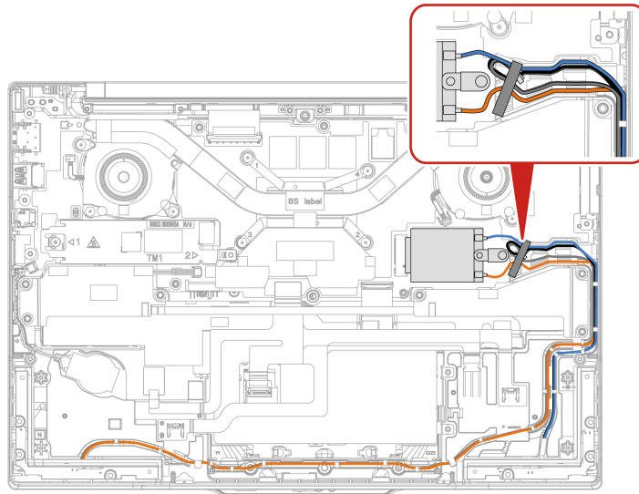
Type two – 4G wireless WAN module with 4 connectors
